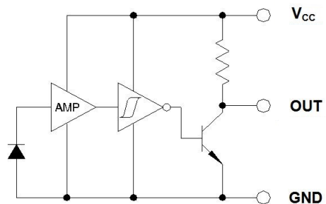
OPL531A OPL536A Inverted 10K Pull-Up
