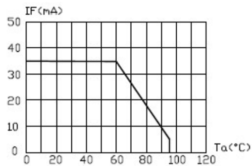
Maximum Forward DC Current vs Ambient
