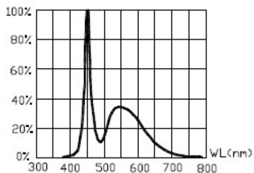
Relative Luminous Flux vs Wavelength
