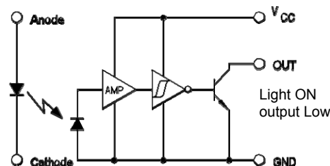
OPB916IOC Inverted Open-Collector
