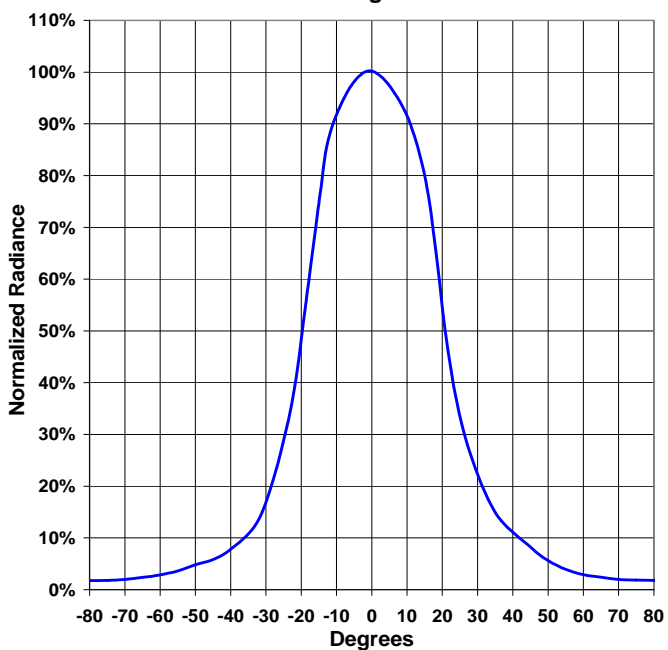
Beam Angle
