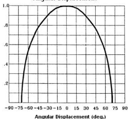
Normalized Collector Current vs. Angular Displacement
