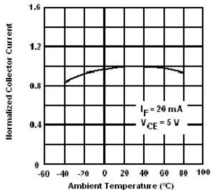
Normalized Collector Current vs. Ambient Temperature
