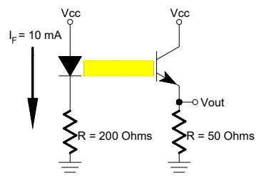
Test Circuit
