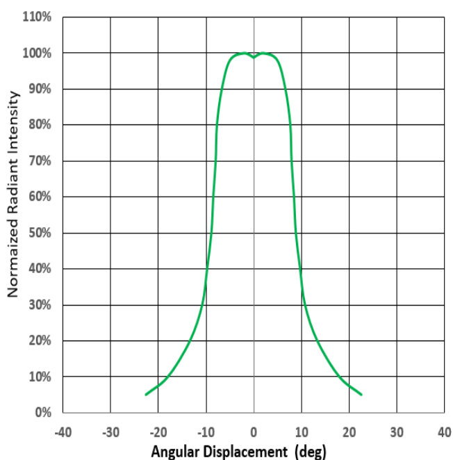
Normalized Radiant Intensity vs Angular Displacement
