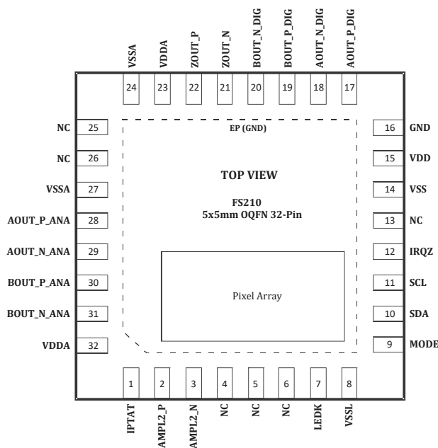
Figure 1: FS210 Pin Configuration (5mm x 5mm QFN - top view)
