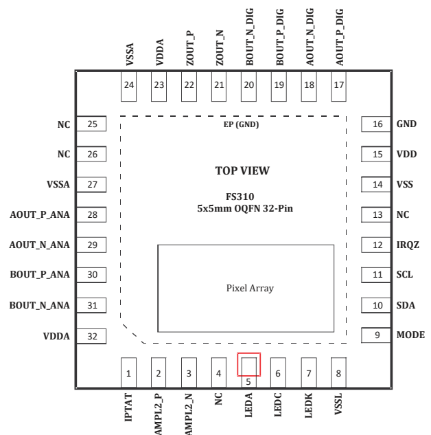
Figure 2: FS310 Pin Configuration (5mm x 5mm QFN - top view)
