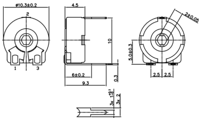
Model 38P (Top Adjust)
