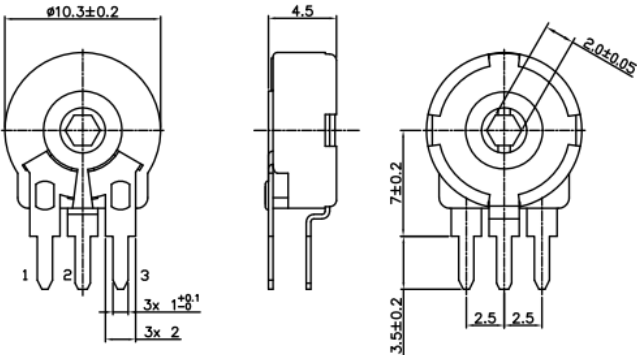
Model 38W (Side Adjust)
