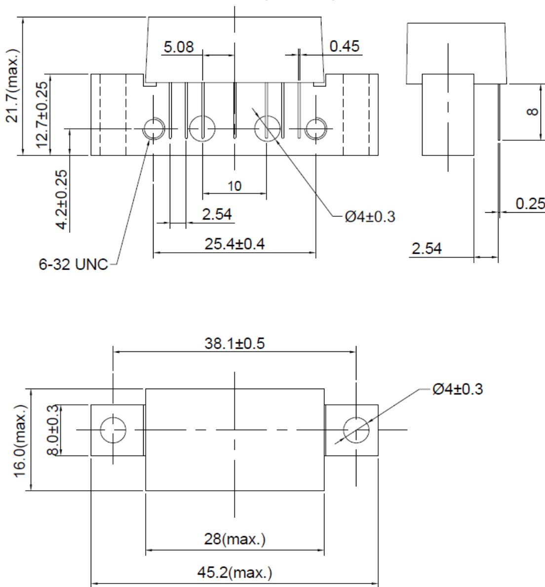
Package Drawing
