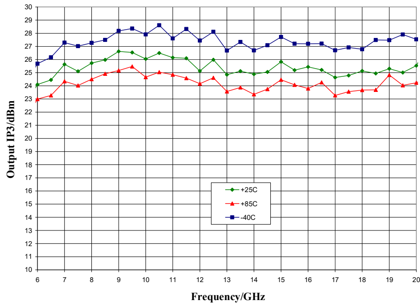
Output IP3 vs. Temperature, V_{dd} = 4.0\text{ V}
