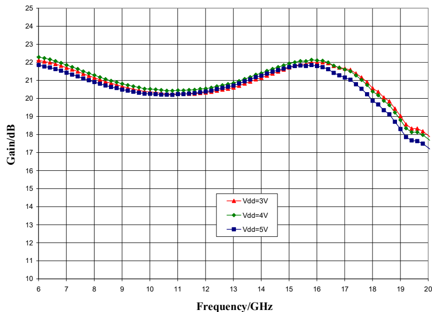
Gain vs. V_{dd} , T_A = 25^\circ\text{C}
