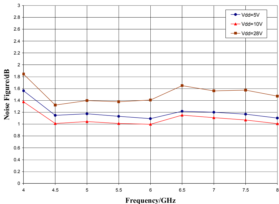
Noise Figure vs. V_{dd} , V_{gg} = -2.3\text{ V} , T_A = 25\text{ °C}
