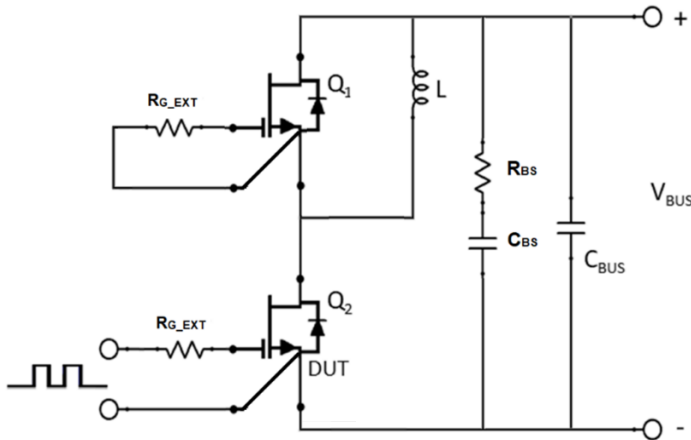
Figure 23. Schematic of the half-bridge mode switching test circuit. Note, a bus RC snubber ( R_{BS} = 2.5\Omega , C_{BS} = 100\text{nF} ) is used to reduce the power loop high frequency oscillations.
