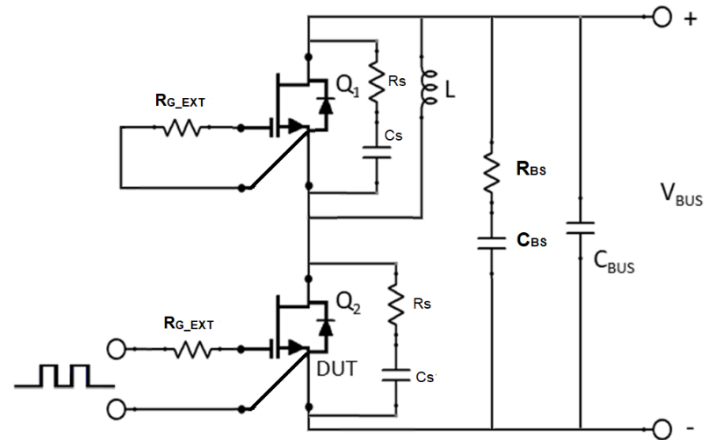
Figure 24. Schematic of the half-bridge mode switching test circuit with device RC snubbers ( R_S = 10\Omega , C_S = 100\text{pF} ) and a bus RC snubber ( R_{BS} = 2.5\Omega , C_{BS} = 100\text{nF} ).
