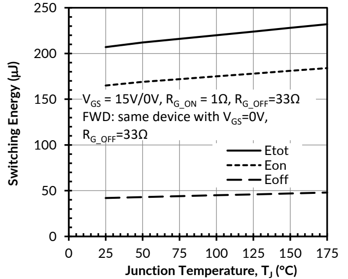
Figure 22. Clamped inductive switching energy vs. junction temperature at V_{DS} = 400\text{V} and I_D = 20\text{A}
