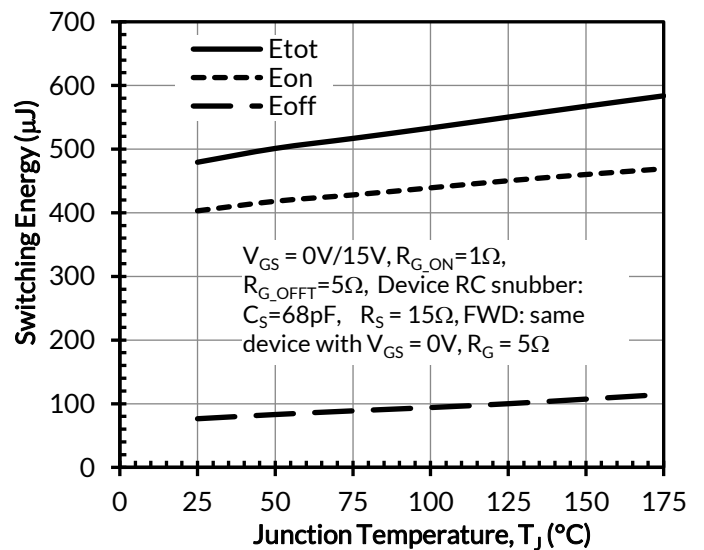
Figure 28. Clamped inductive switching energy vs. junction temperature at V_{DS} = 500\text{V} and I_D = 25\text{A}
