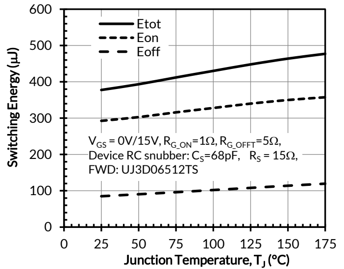
Figure 34. Clamped inductive switching energy vs. junction temperature at V_{DS} = 500\text{V} and I_D = 25\text{A}
