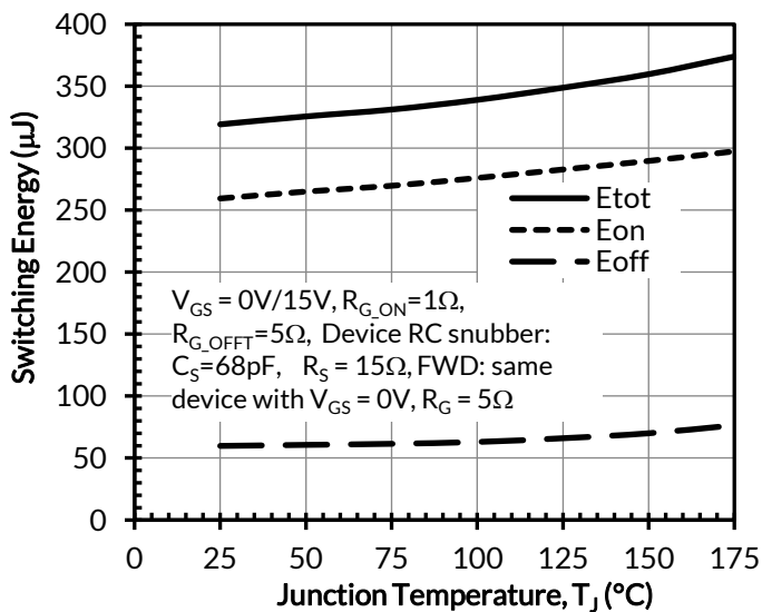
Figure 27. Clamped inductive switching energy vs. junction temperature at V_{DS} = 400\text{V} and I_D = 25\text{A}
