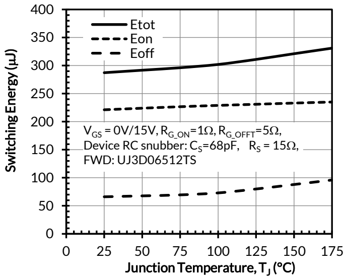
Figure 33. Clamped inductive switching energy vs. junction temperature at V_{DS} = 400\text{V} and I_D = 25\text{A}
