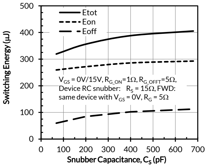
Figure 25. Clamped inductive switching energies vs. snubber capacitance C_S at V_{DS} = 400\text{V} , I_D = 25\text{A} , and T_J = 25^\circ\text{C}
