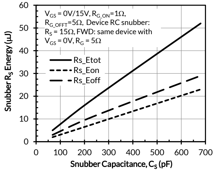
Figure 26. RC snubber energy losses vs. snubber capacitance C_S at V_{DS} = 400\text{V} , I_D = 25\text{A} , and T_J = 25^\circ\text{C}
