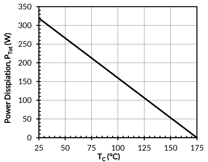
Figure 4. Power dissipation
