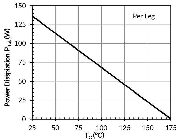
Figure 4. Power dissipation
