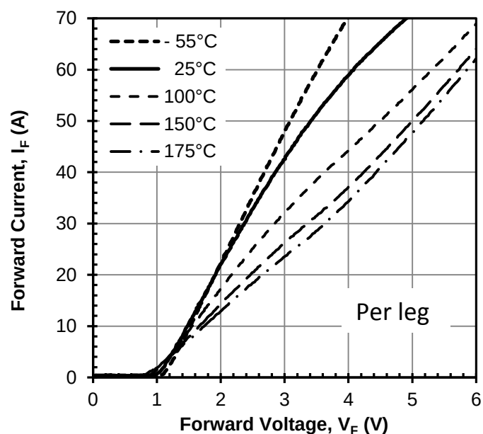
Figure 2 Typical forward characteristics in surge current per leg
