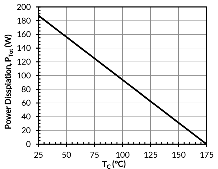
Figure 4. Power dissipation
