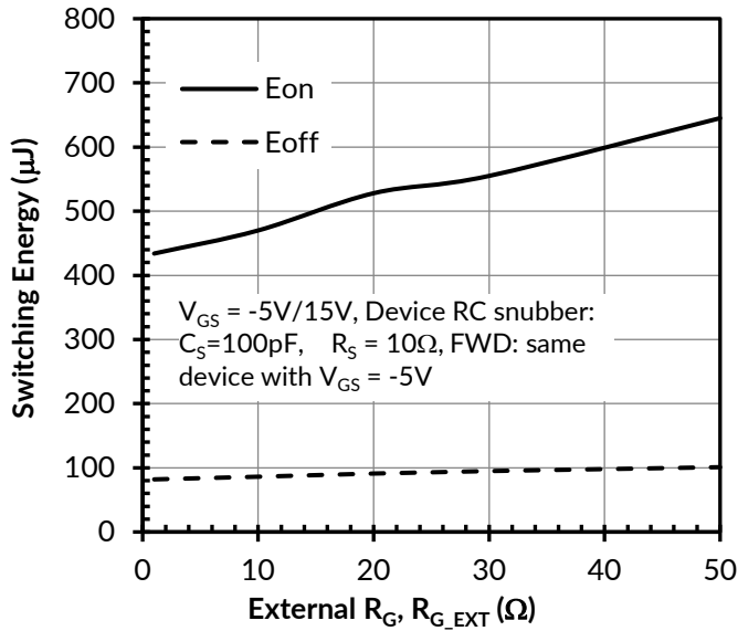
Figure 21. Clamped inductive switching energies vs. R_{G\_EXT} at V_{DS} = 800\text{V} , I_D = 30\text{A} , and T_J = 25^\circ\text{C}
