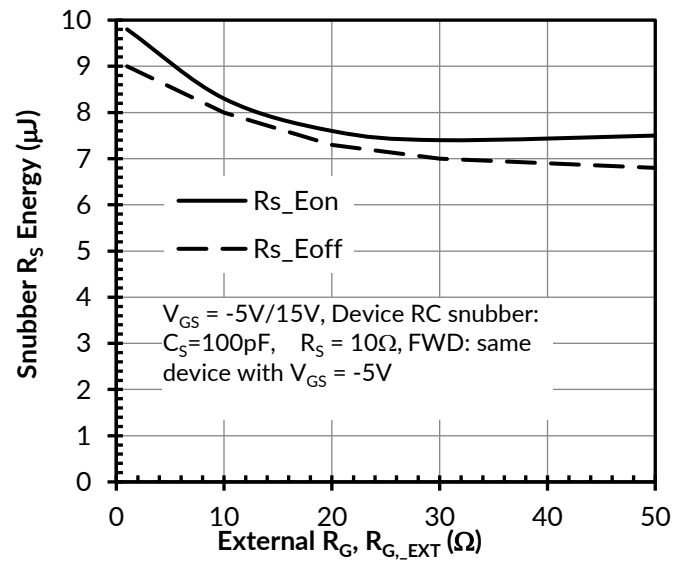
Figure 22. RC snubber energy losses vs. R_{G\_EXT} at V_{DS} = 800\text{V} , I_D = 30\text{A} , and T_J = 25^\circ\text{C}
