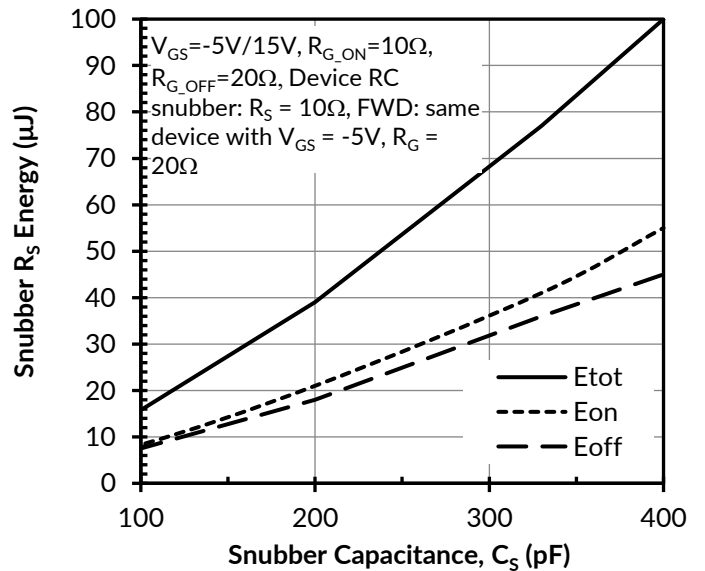
Figure 24. RC snubber energy losses vs. snubber capacitance C_S at V_{DS} = 800\text{V} , I_D = 30\text{A} , and T_J = 25^\circ\text{C}
