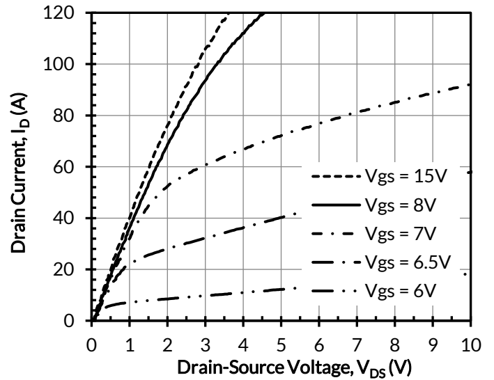
Figure 2. Typical output characteristics at T_j = 25^\circ\text{C} ,
