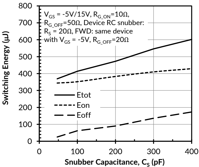
Figure 23. Clamped inductive switching energies vs. snubber capacitance C_S at V_{DS} = 800V , I_D = 20A , and T_J = 25^\circ\text{C}
