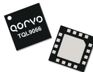
16-pin 4x4 mm QFN Package
