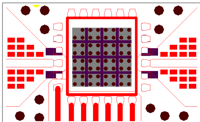
Via pattern
