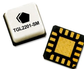
QFN 3 x 3 mm 16 L Package
