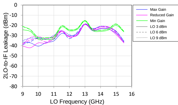
LSB 2LO-to-IF Leakage vs. LO Freq vs. LO Power and State
