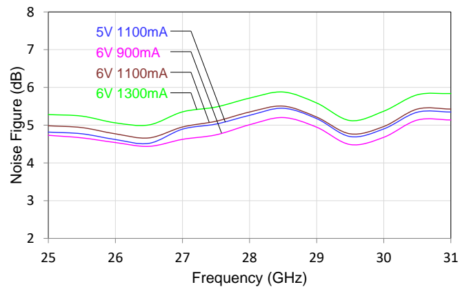
Noise vs. Frequency vs. Bias
