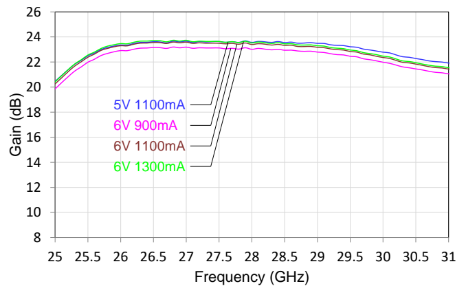
Gain vs. Frequency vs. Bias
