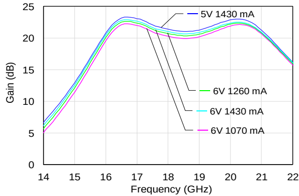
Gain vs. Frequency vs. Bias
