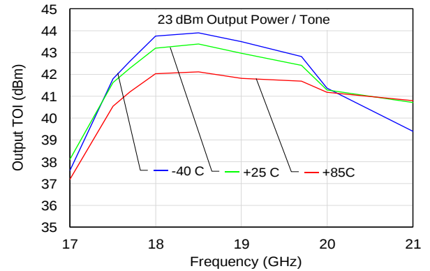
Output TOI vs. Frequency vs. Temperature
