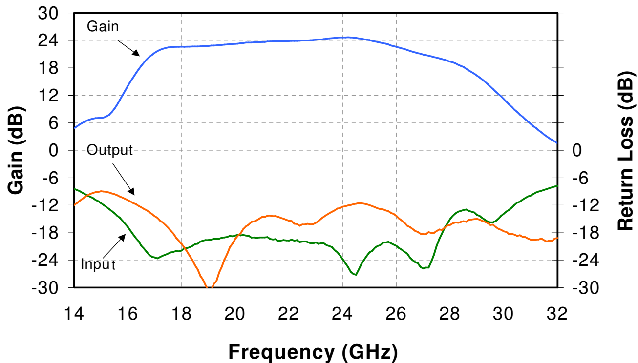
Measured Fixtured Data Bias Conditions: V_d = 7\text{ V} , I_d = 760\text{ mA}
