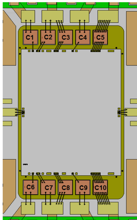
MMIC mounting/wire bonding detail
