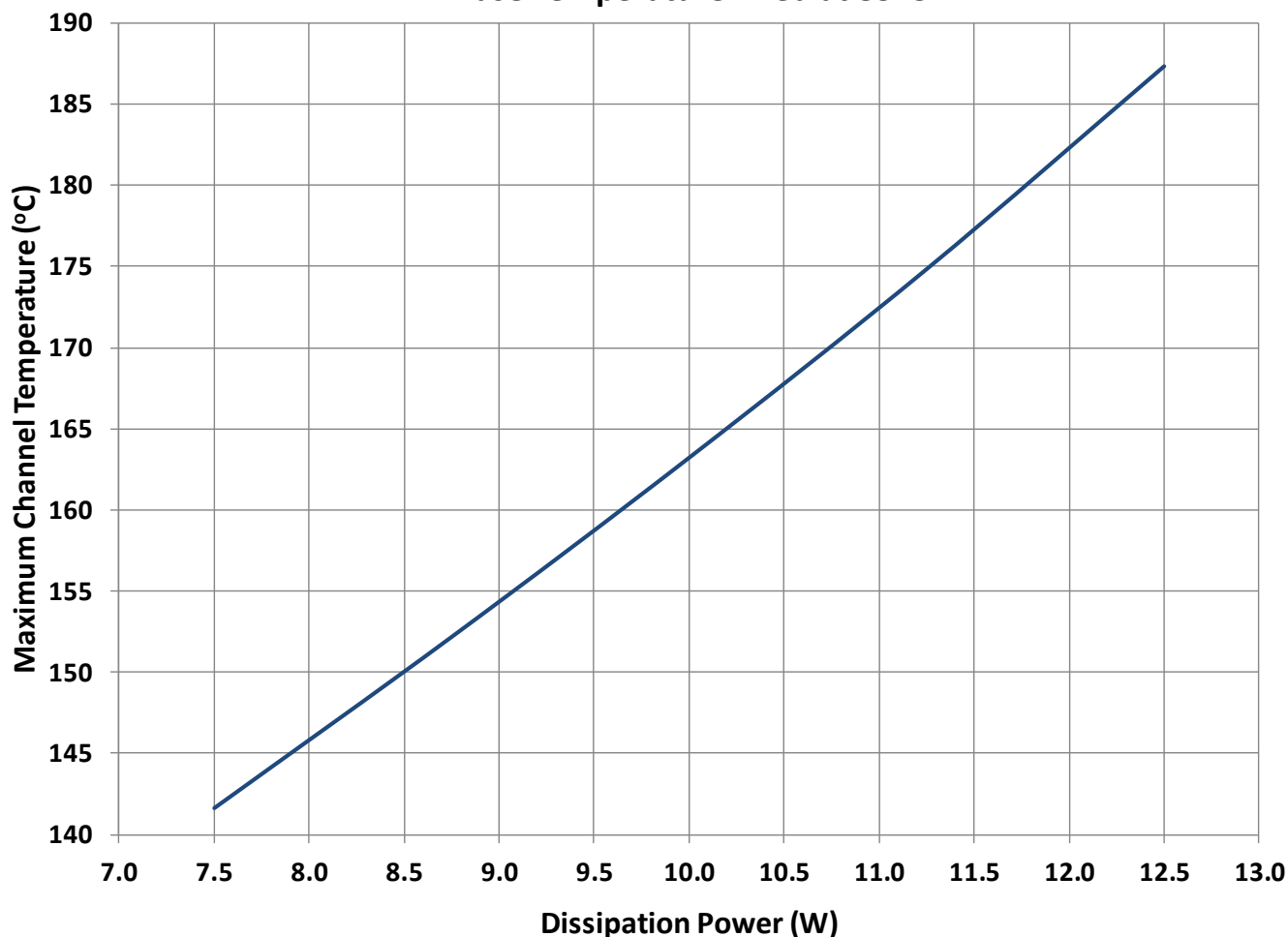
Peak IR Surface Temperature vs. Dissipation Power Base Temperature Fixed at 85°C
