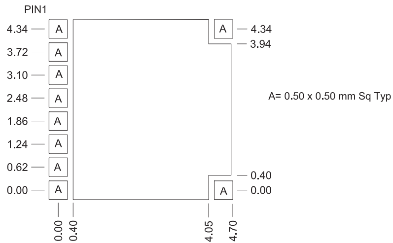
SOLDER MASK PATTERN
