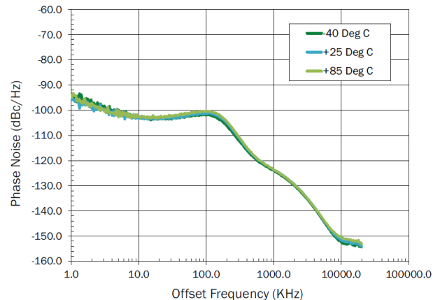
Synthesizer Phase Noise vs Temperature 1500MHz LO Frequency, 26MHz TCXO
