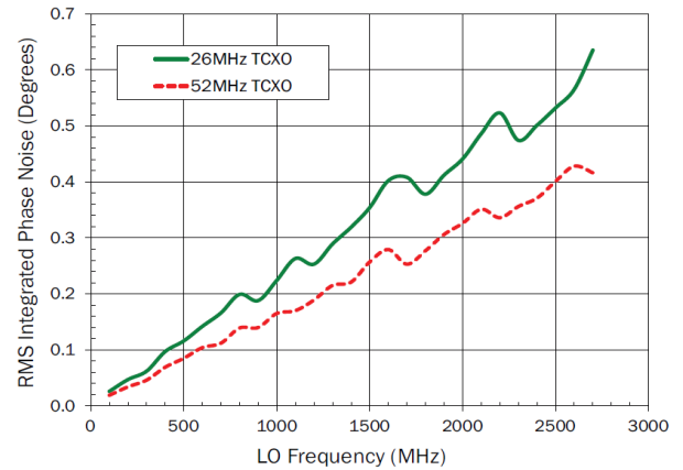
Synthesiser RMS Integrated Phase Noise Integration Bandwidth 1KHz to 40MHz
