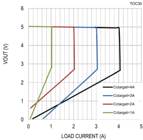
Figure 41. Main-buck Constant Current
