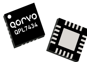
20 Pad 4.0 x 4.0 x 0.85 mm QFN Package
