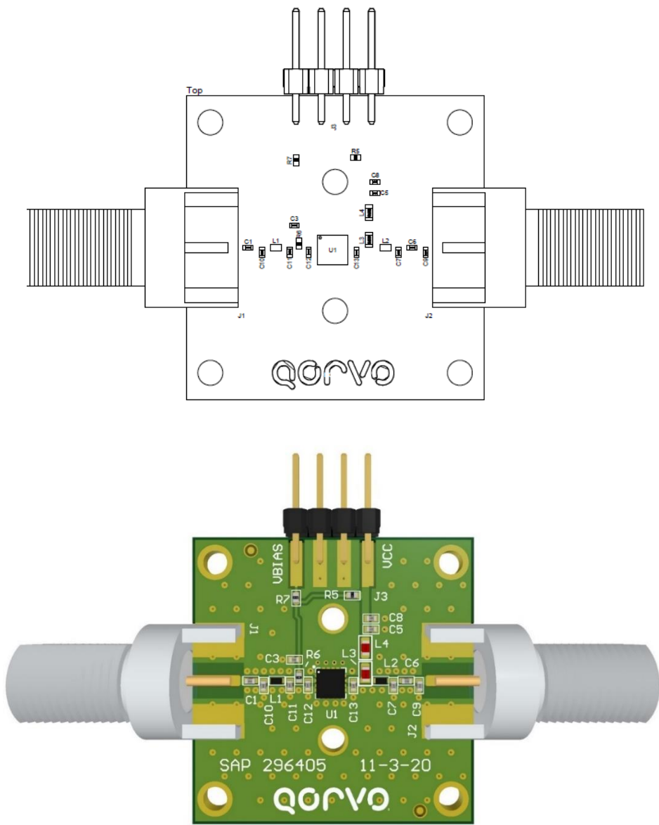
QPL1819 Evaluation Board
