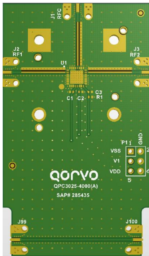
Layout
