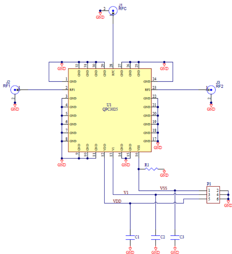
Schematic
