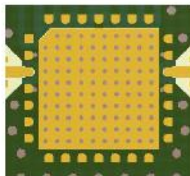
MOUNTING DETAIL
