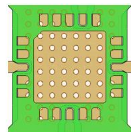
Mounting Pads Details
