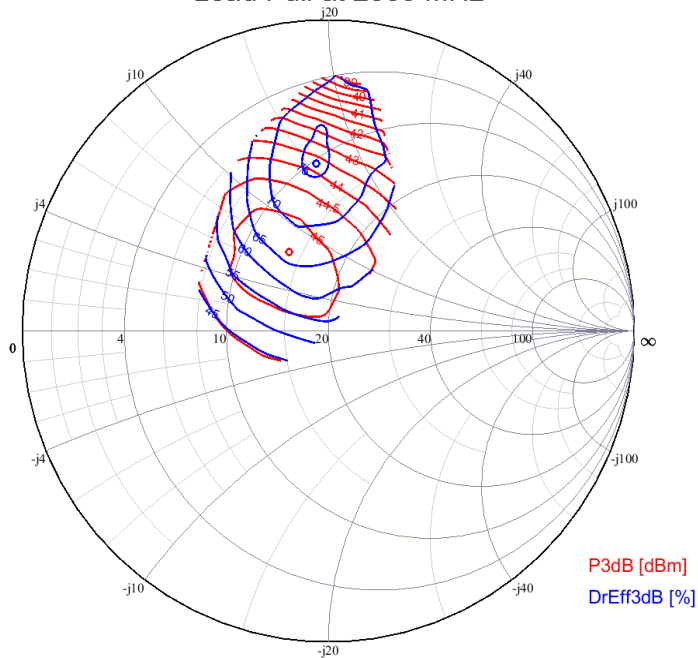
Load Pull at 2600 MHz
