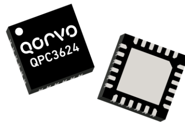
24 Pad 4 x 4 mm QFN Package
