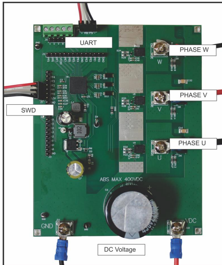
Figure 7: PAC5556AEVK3 Evaluation Module Connections
