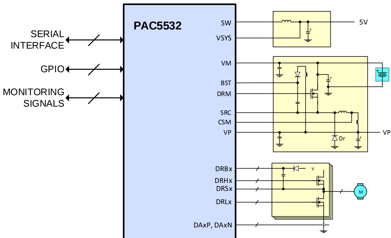
Figure 25-1 3-Phase Motor Using PAC5532 (Simplified Diagram)
