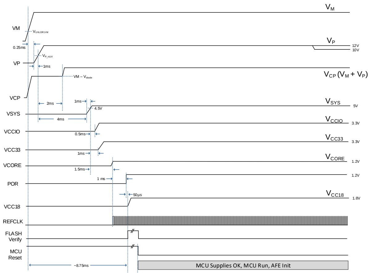
Figure 5 Power-up Sequence
