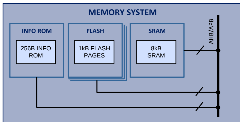
Figure 15-1 Memory System
