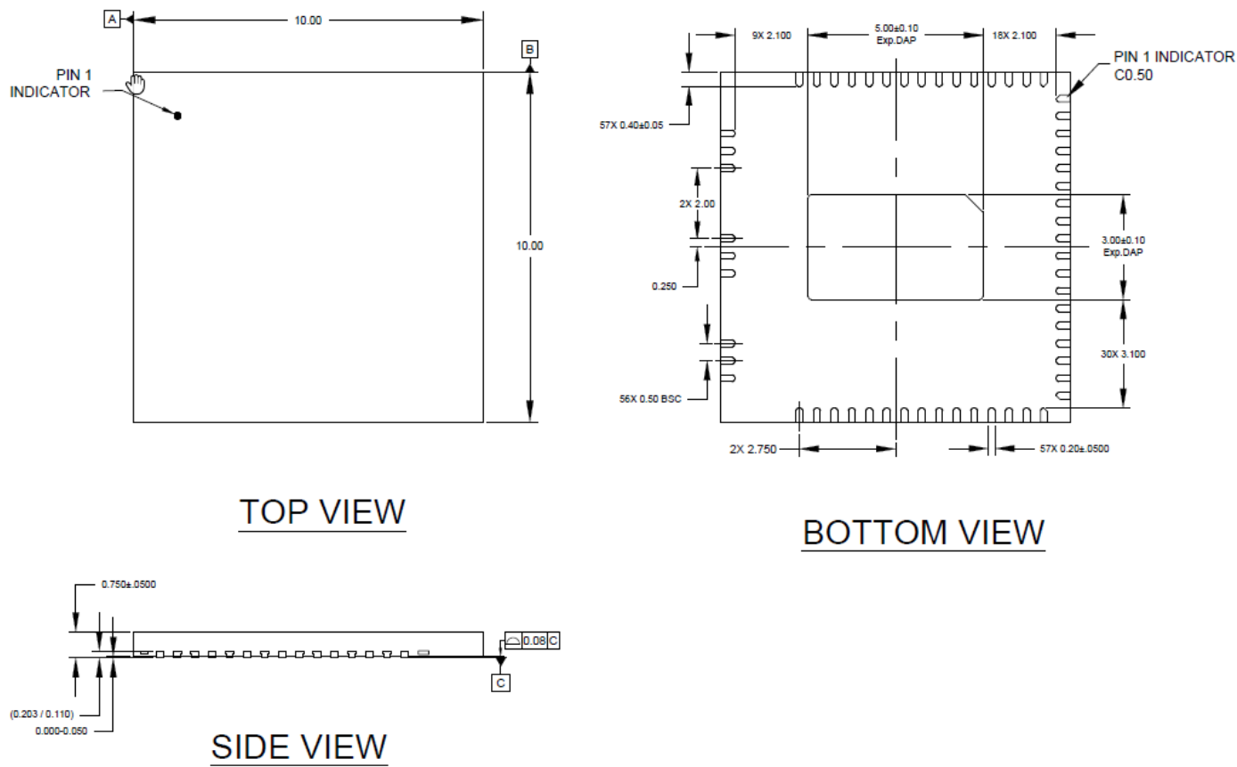
Figure 22-1 TQFN1010-57
