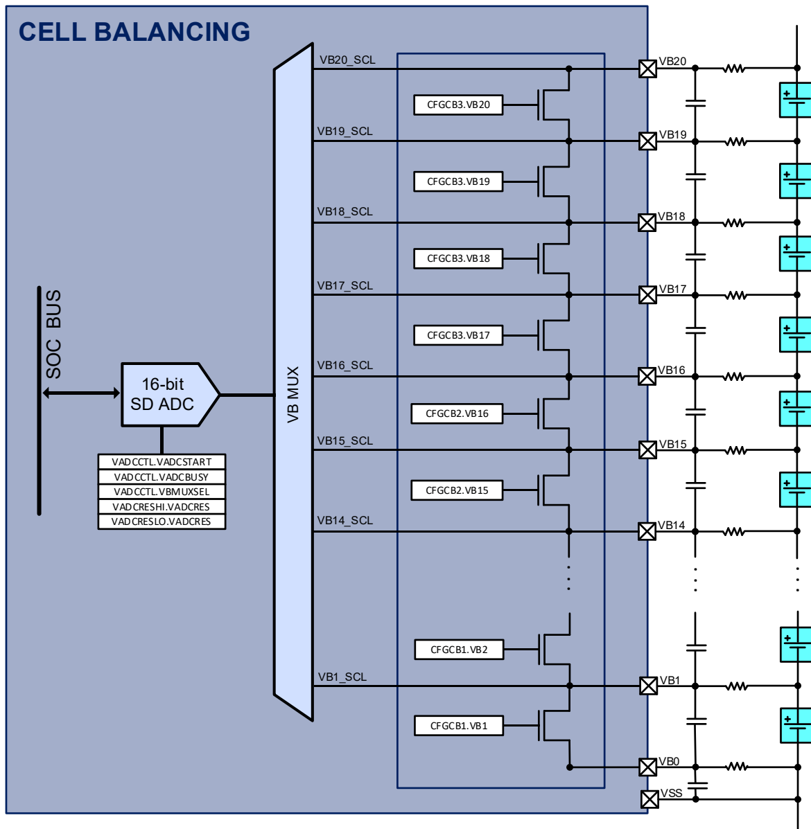
Figure 14 Cell Balancing
