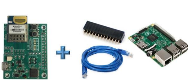
Figure 2: The module development board can be used to create an Anchor, a Tag or a Gateway
