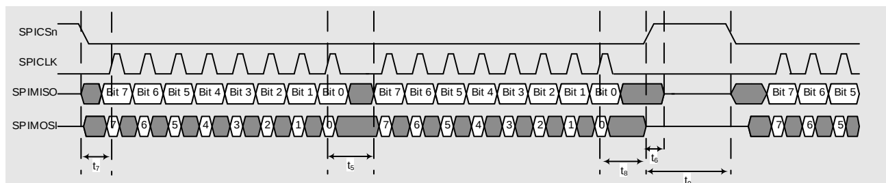
Figure 13: SPI Timing Diagram
