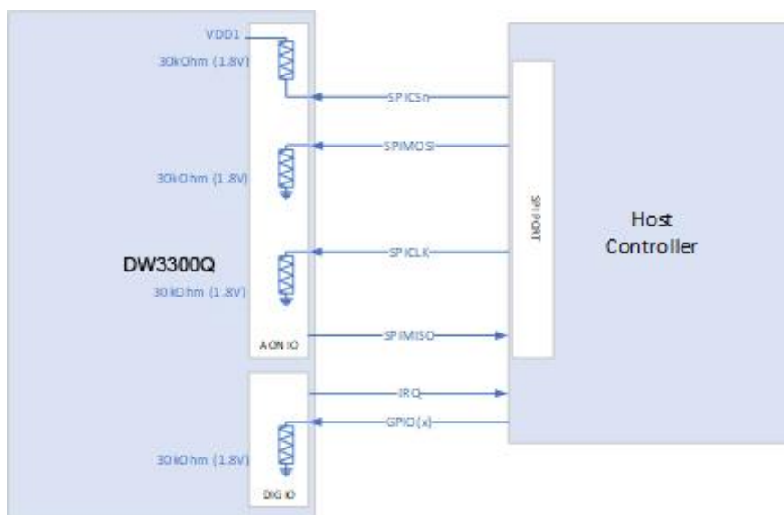
Figure 18: SPI and GPIO Pull Up/Down
