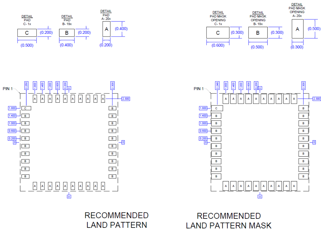
Figure 34: Package Dimensions LGA
