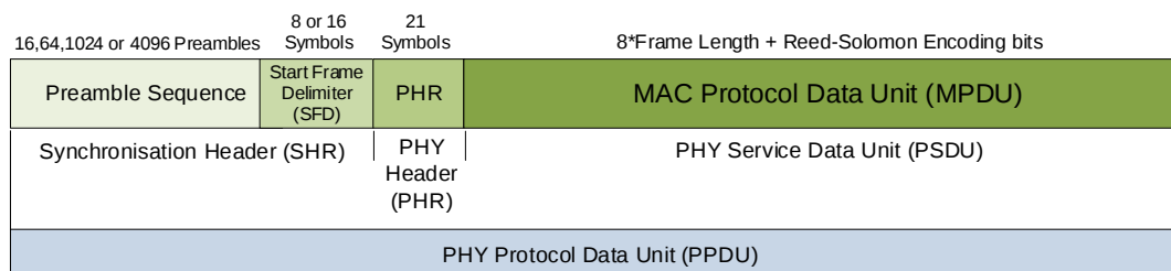
Figure 11: IEEE802.15.4-2011 PPDU Structure
