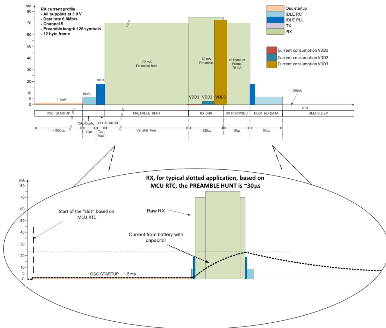
Figure 29: Typical Current Profiles When Receiving a Frame for Different Types of Applications
