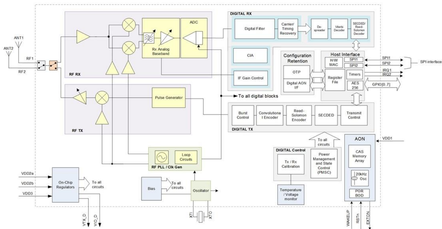
Figure 1: Block Diagram
