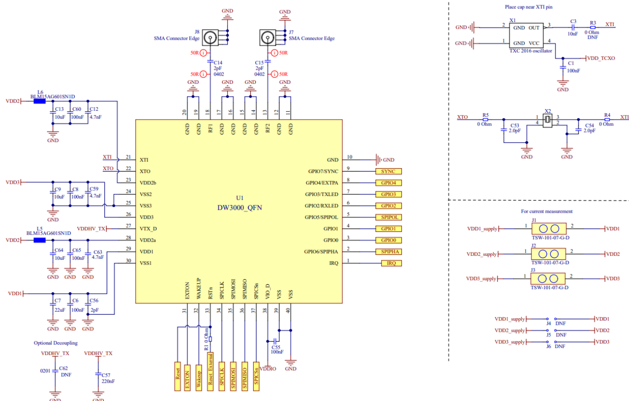
Figure 33: EVB Circuit Diagram
