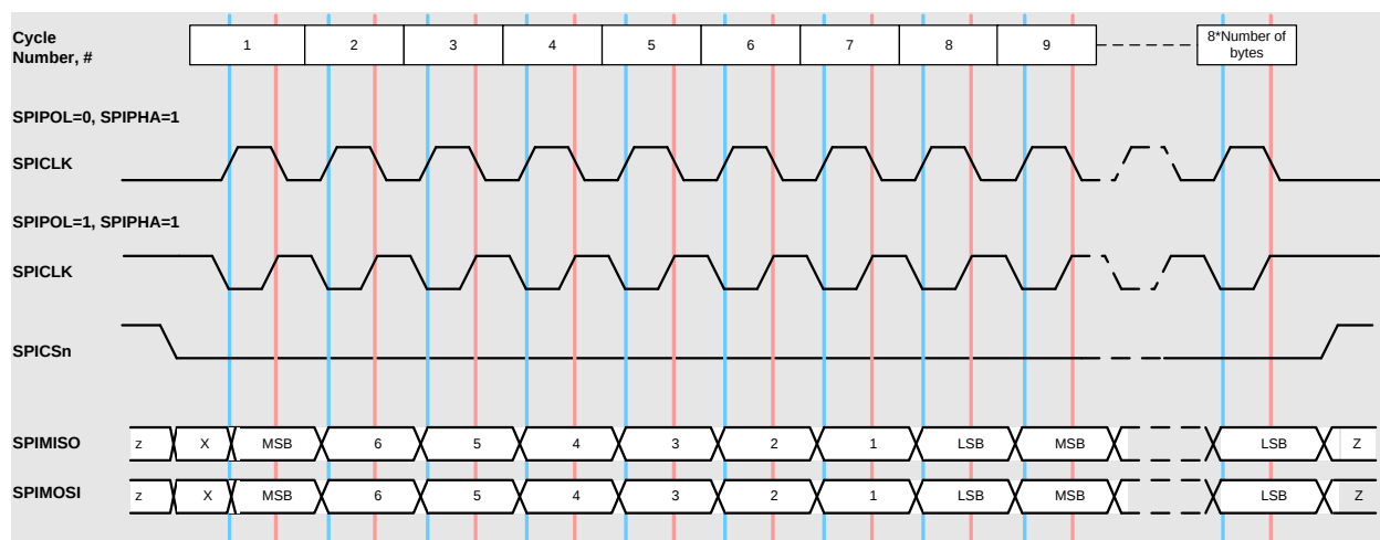
Figure 16: DW3300Q SPIPHA=1 Transfer Protocol
