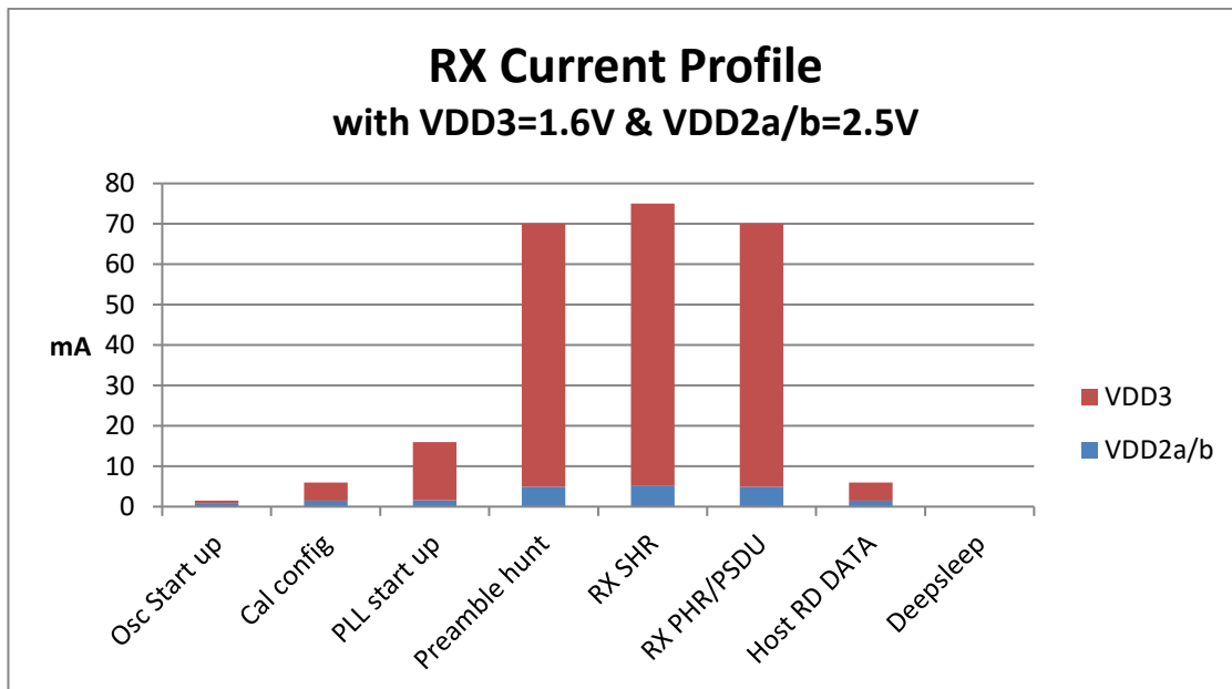
Figure 30: Current Consumption During RX for High Efficiency Powering Modes
