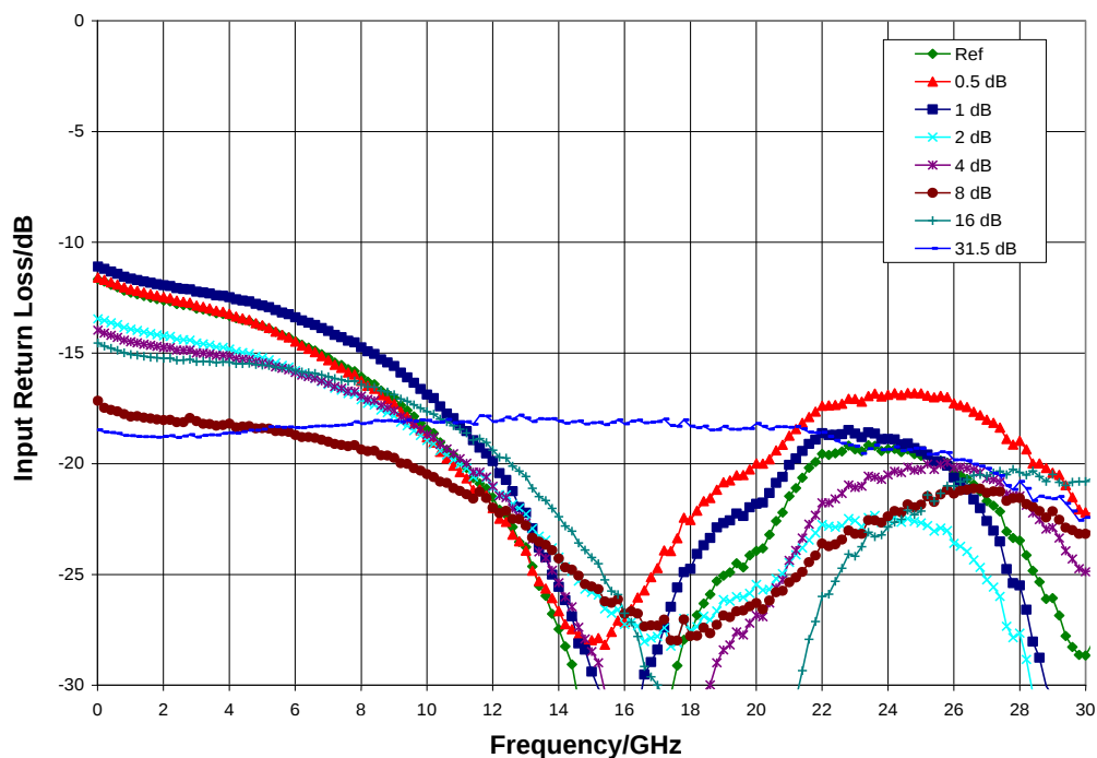
Input Return Loss (major states only), T_A = 25^\circ\text{C}
