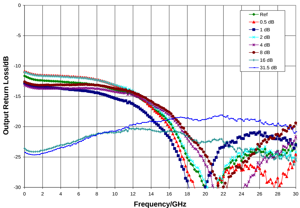
Output Return Loss (major states only), T_A = 25^\circ\text{C}
